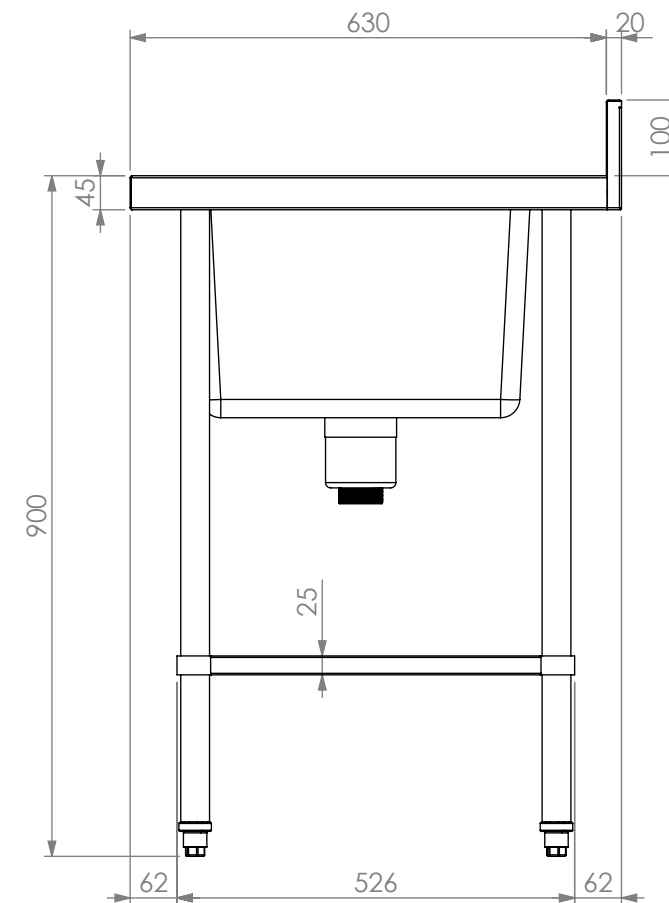
SIDE ELEVATION
